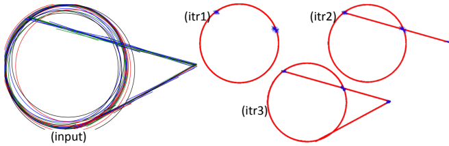
Figure 3: This figure shows steps of the method. It starts with an over-generation of primitives and at each iteration adds a primitive that provides the biggest gain based on Equation 4. Red line segments correspond to primitives that are added at each iteration. Blue crosses correspond to detected corners.
